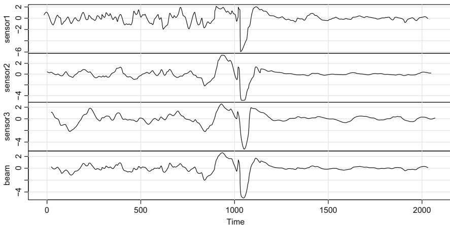
Fig. 7.6. Three series for a nuclear explosion detonated 25 km south of Christmas Island and the delayed average or beam. The time scale is 10 points per second
