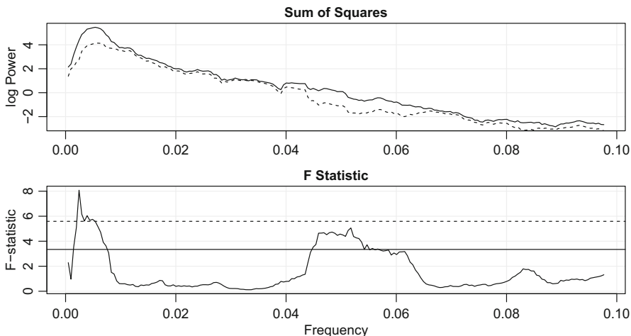
Fig. 7.7. Analysis of power for infrasound array on a log scale ( top panel ) with SST(\omega) shown as a solid line and SSE(\omega) as a dashed line . The F -statistics ( bottom panel ) showing detections with the dashed line based on an FDR level of .001 and the solid line corresponding null F quantile
